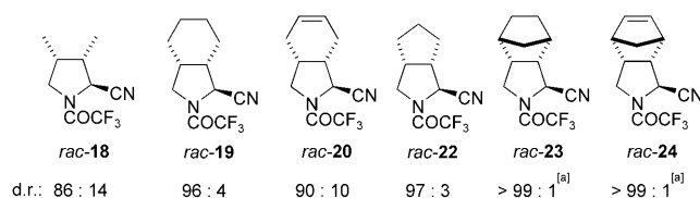
Figure 5. Diastereoselectivity of HCN addition for racemic samples with TMSCN/MeOH in CH 2 Cl 2 as determined by GC-FID ( 18–22 ) in the crude products. [a] Only one diastereomer was detected by NMR spectroscopy (free amino nitrile) and GC-MS.
